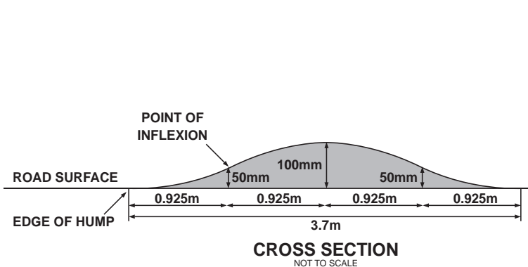
Fig 4.7 Cross-section and plan view of a sinusoidal hump
