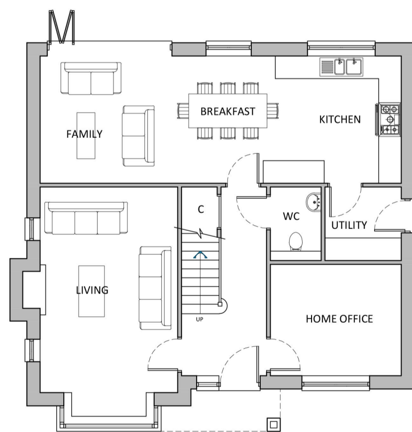
PLOT 15 GROUND FLOOR PLAN
