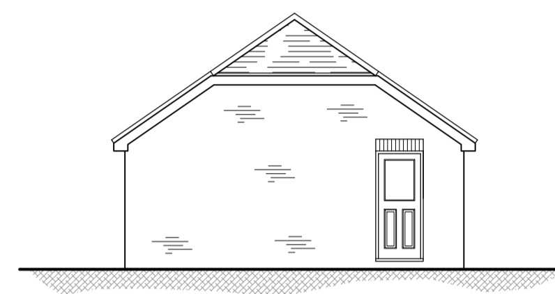
SIDE ELEVATION
