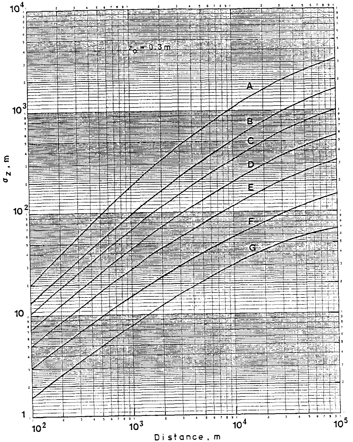
Figure 8. Vertical standard deviation, \sigma_z , as a function of distance for each Pasquill stability category and a ground roughness length of 0.3 m
