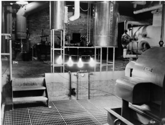
FIG. 2.4. Light bulbs at Idaho Falls, USA powered by steam generated by a nuclear reactor (reproduced with permission courtesy of the Idaho National Laboratory, USA).
