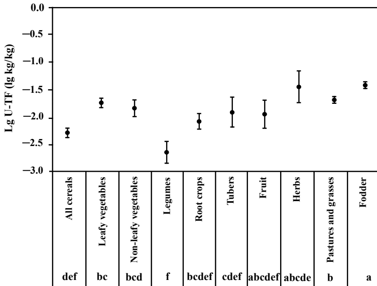
FIG. 6.4. Logarithm of uranium soil to plant transfer factor (TF) values (kg/kg, dry weight) for different crop groups (adapted from Ref. [6.37]). The error bars denote residual standard error after analysis of variance accounting for the effect of plant type. Transfer factors for crop groups assigned the same letter are not significantly different ( p < 0.05 ).
