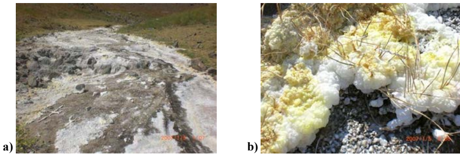
FIG. 9.6. (a) Acidic seepage water from the tailings body; (b) precipitate residues of sodium sulphate with uranium incorporated (photographs from Taboshar, Tajikistan, taken by O. Voitsekho vych, Ukrainian Hydrometeorological Institute).
