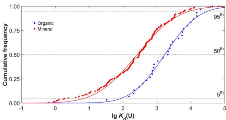
FIG. 6.2. Cumulative distribution functions of K_d(U) for mineral and organic groups.
